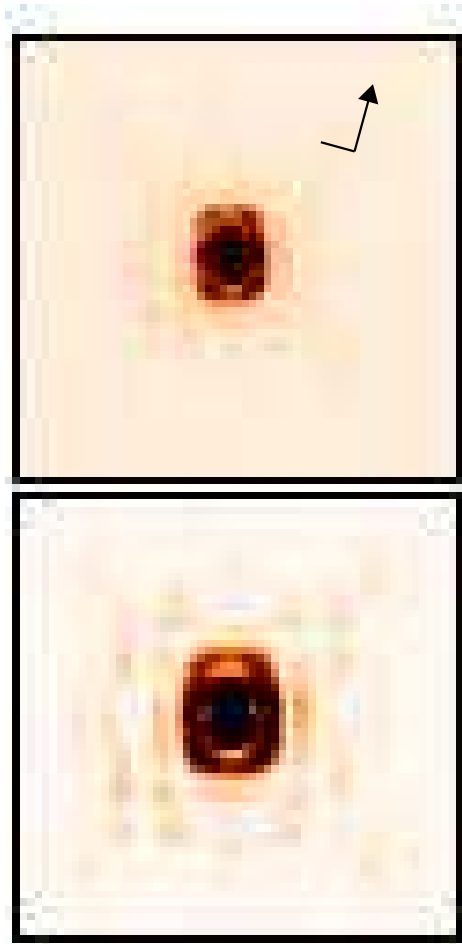
FIG. 1.— HST NICMOS F110W (top) and F170M (bottom) observations of the binary SDSS 0423–0414AB. Images are 2''5 on a side, and orientation is given by the compass in the top panel indicating north (arrow) and east.
